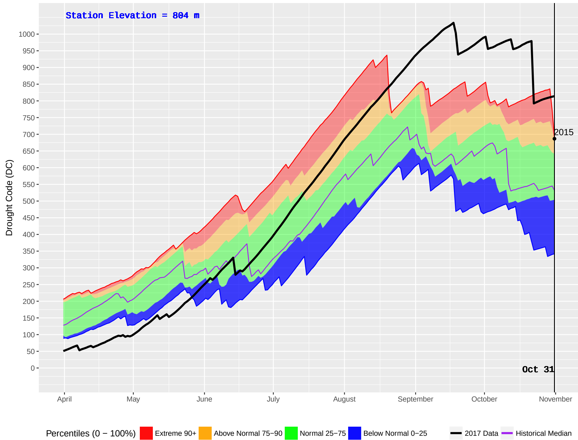
KOOCANUSA (1075) : Historical (2010–2016) and Current (2017) Noon Drought Code (DC)
