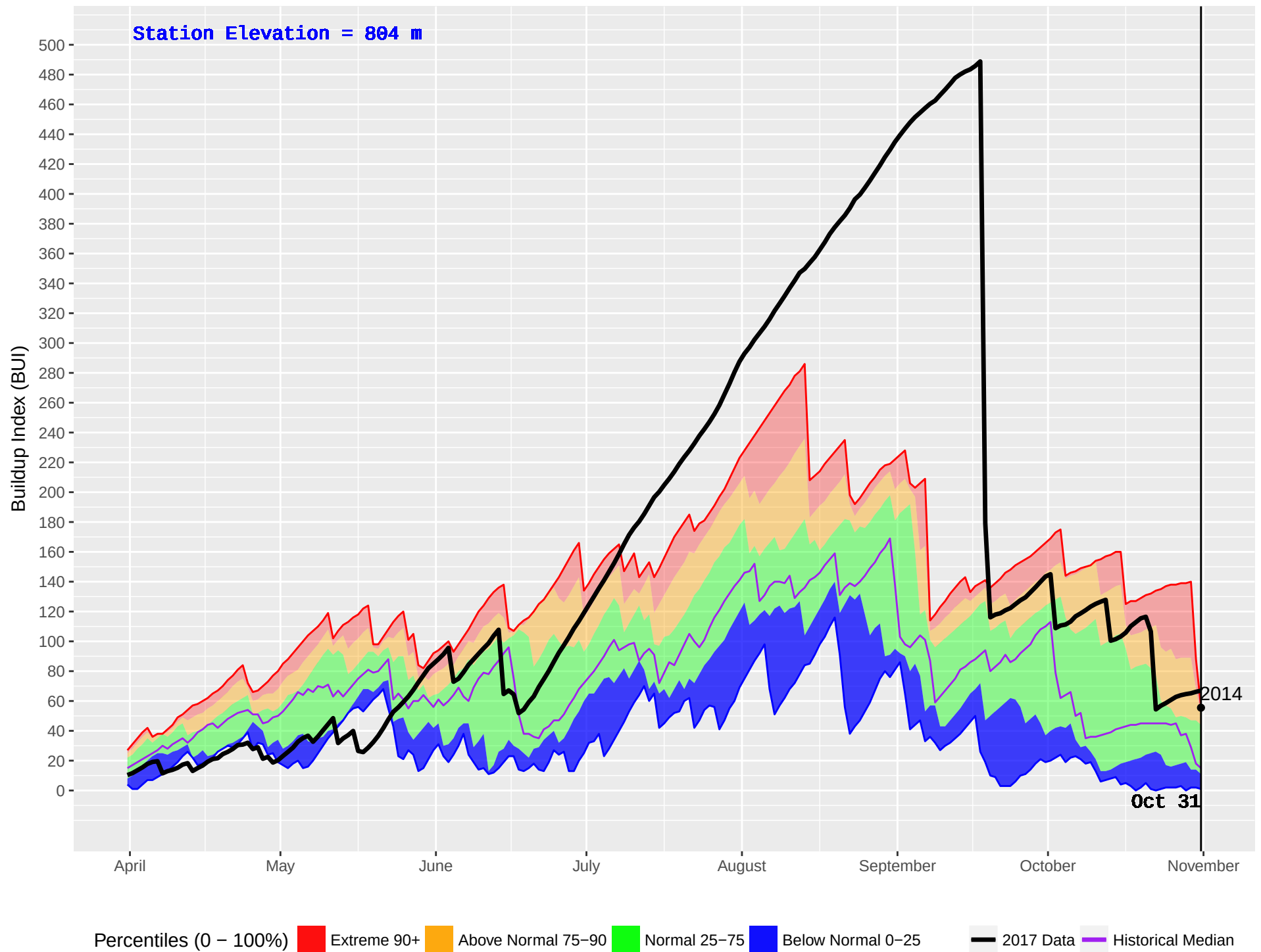
KOOCANUSA (1075) : Historical (2010–2016) and Current (2017) Noon Buildup Index (BUI)
