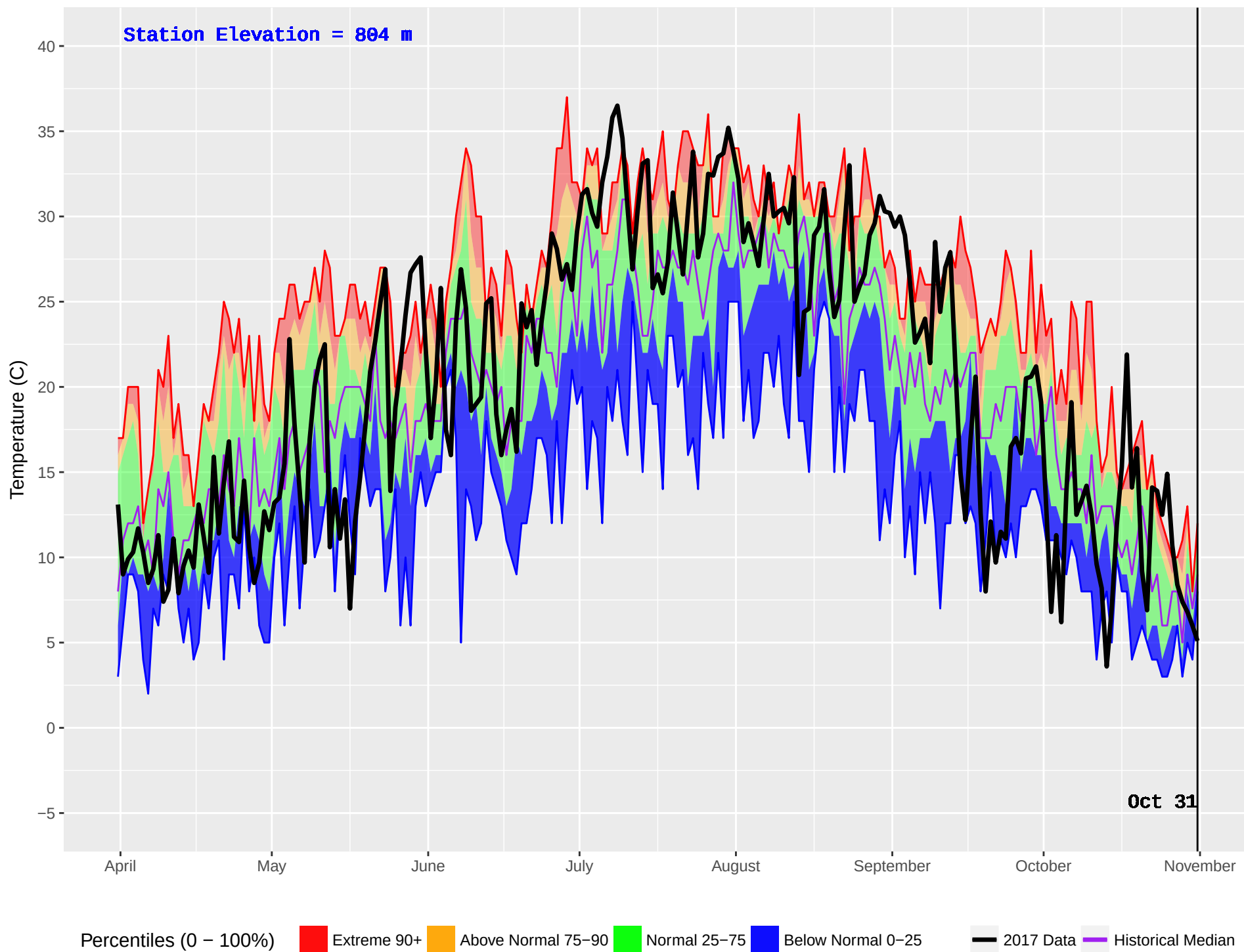
KOOCANUSA (1075) : Historical (2010–2016) and Current (2017) Noon Temperature
